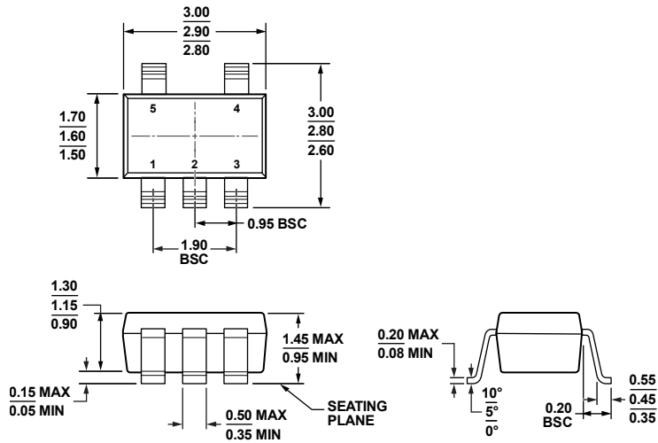
Figure 50. 5-Lead Small Outline Transistor Package [SOT-23] (RJ-5)
