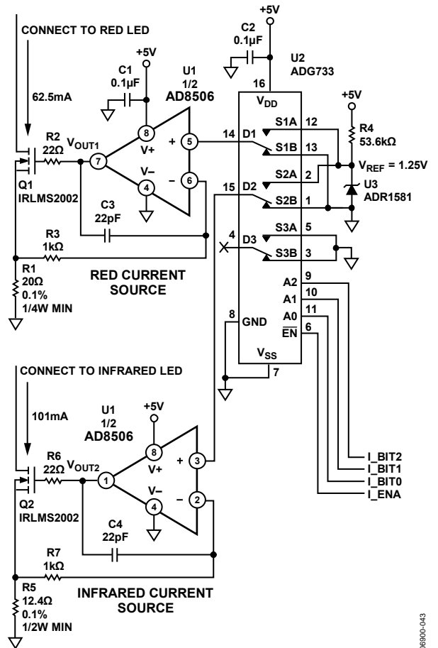
Figure 48. Pulse Oximeter Red and Infrared Current Sources Using the AD8506 as a Buffer to the Voltage Reference Device
