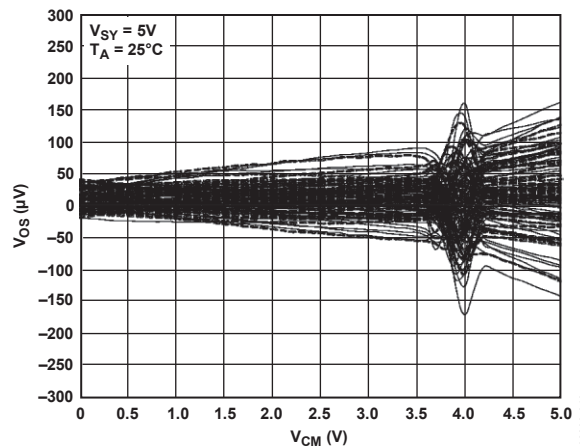
Figure 45. Typical Input Offset Voltage vs. Common-Mode Voltage Response in a Dual Differential Pair Input Stage Op Amp (Powered by 5 V Supply; Results of Approximately 100 Units per Graph Are Displayed)
