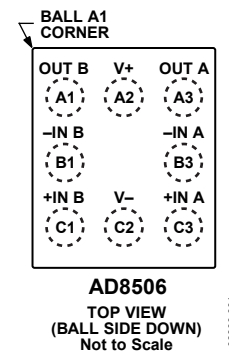
Figure 3. 8-Ball WLCSP (CB-8-2)
