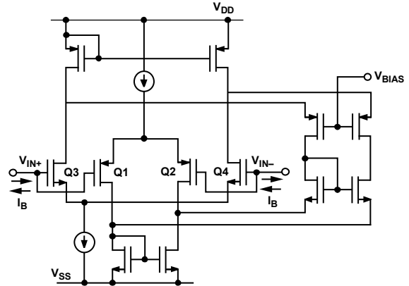
Figure 44. A Typical Dual Differential Pair Input Stage Op Amp (Dual PMOS Q1 and Q2 Transistors Form the Lower End of the Input Voltage Range, Whereas Dual NMOS Q3 and Q4 Compose the Upper End)
