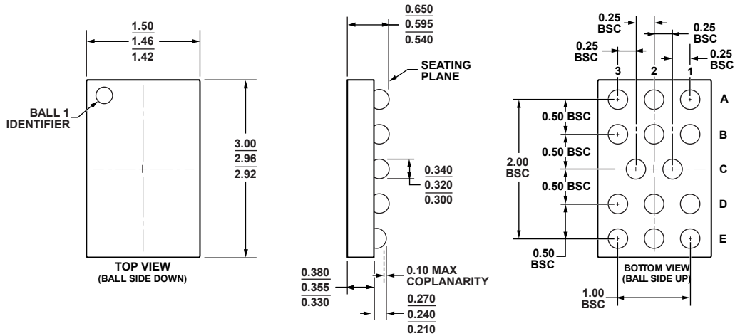
Figure 54. 14-Ball Wafer Level Chip Scale Package [WLCSP] (CB-14-1) Dimensions shown in millimeters
