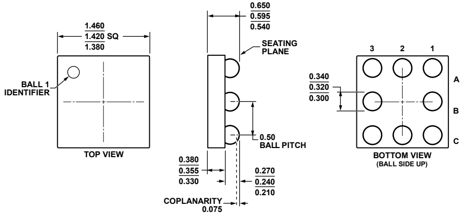
Figure 52. 8-Ball Wafer Level Chip Scale Package [WLCSP] (CB-8-2) Dimensions shown in millimeters
