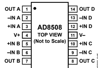
Figure 4. 14-Lead TSSOP (RU-14)
