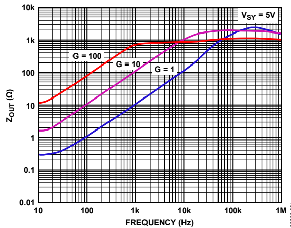
Figure 29. Z_{OUT} vs. Frequency
