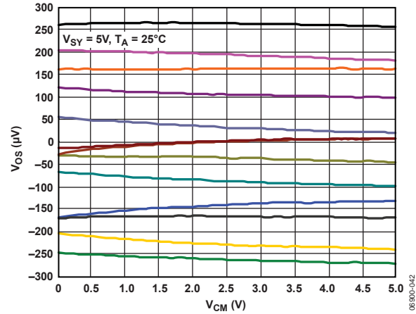
Figure 47. Input Offset Voltage vs. Input Common-Mode Voltage Response (Powered by a 5 V Supply; Results of 12 Units Are Displayed)
