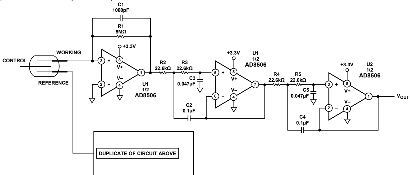
Figure 49. A Four-Pole Butterworth Filter That Can Be Used in a Glucose Meter
