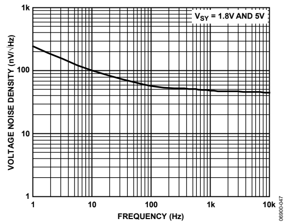
Figure 41. Voltage Noise Density vs. Frequency
