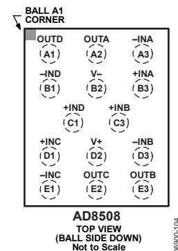
Figure 5. 14-Ball WLCSP (CB-14-1)
